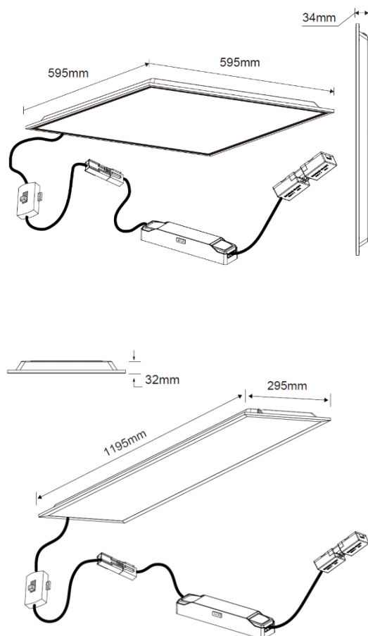
Dimension Diagram
